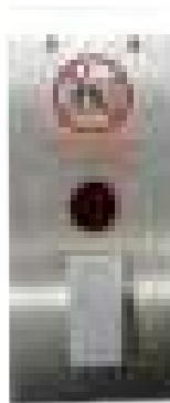
No-entry & Fire-alarm recall key switch (EN81.73)
